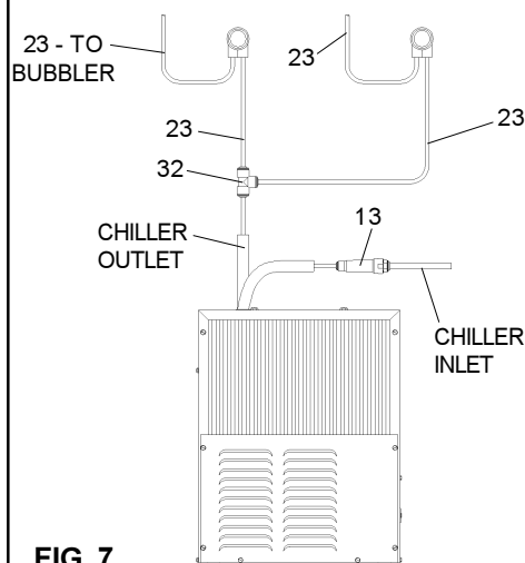
ERFP28C/ERFP28RAC TUBE ROUTING
