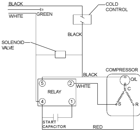
WIRING DIAGRAM
